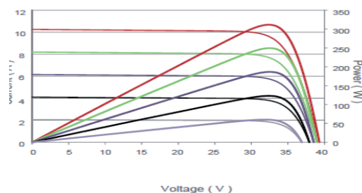
Current-Voltage & Power-Voltage Curves (310W)
