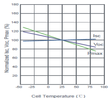
Temperature Dependence of Isc, Voc, Pmax
